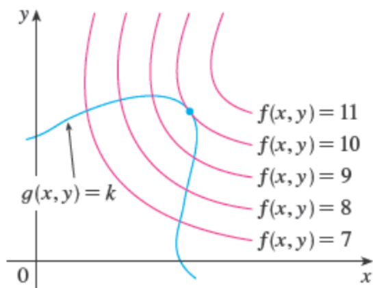
Figure 3.0.1: Maximizing f(x, y) subject to g(x, y) = k
