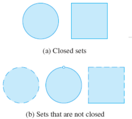
Figure 1.0.2: Closed sets and not closed sets
